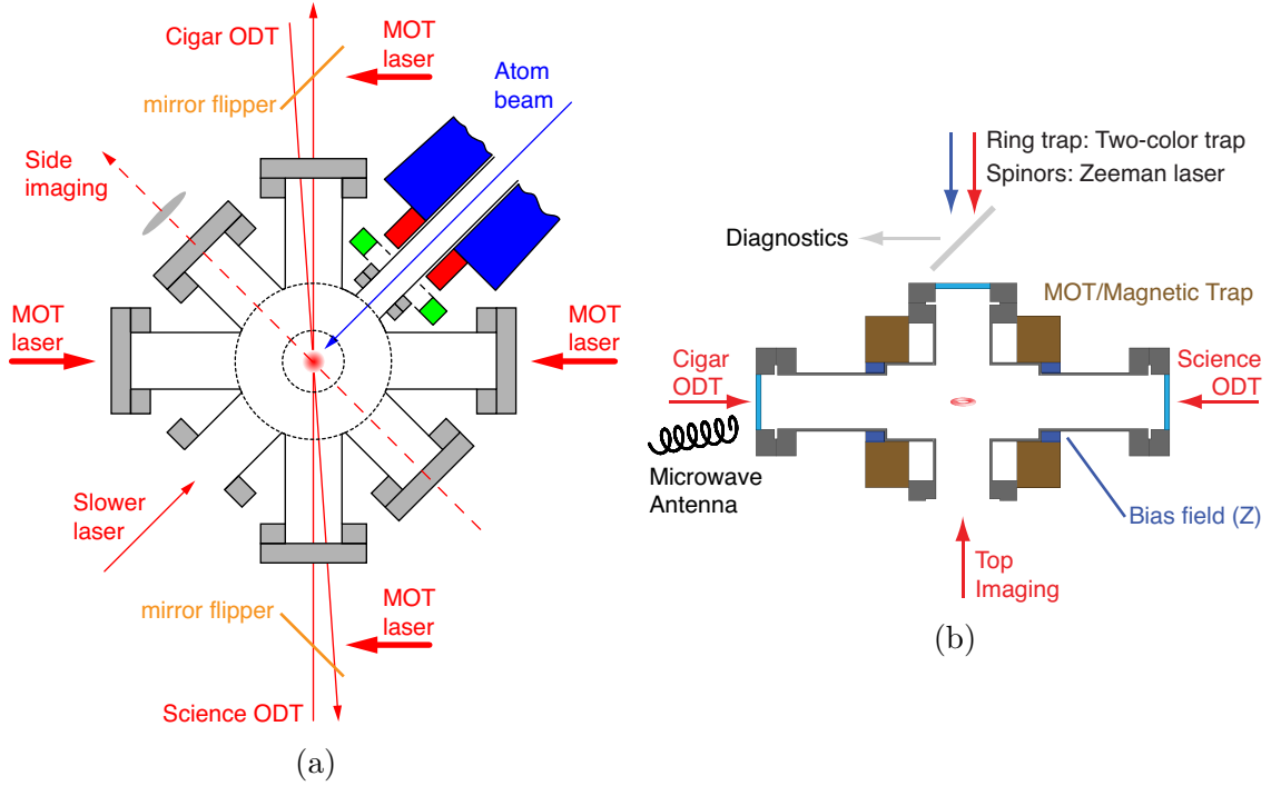
Figure 2.8: MOT/Science chamber layout. (a) Top view shows the four cooling lasers for the MOT and two free-running optical dipole traps (cigar and science ODT). The mirror flippers reflect the MOT lasers during the beginning of the sequence and move out of the way once the atoms are magnetically trapped. (b) Side view shows the microwave antenna and vertical optics. Not shown are the vertical cooling (MOT) lasers.
