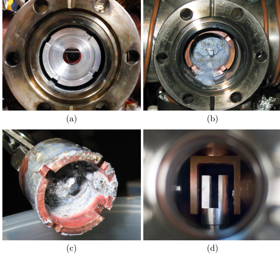
Figure 2.6: Cold catcher cup, (a) empty and (b-c) very full. Most of the rubidium atoms ( >99\% ) that leave the oven stick to the cup. It can be removed by unscrewing it with a tool that slips into the four grooves around the cup. When exposed to air, the rubidium changes color, heats up, and flows, which makes the cold catcher cup runneth over. (d) The shutter assembly seen from the top. The cold catcher cup is visible to the right.
