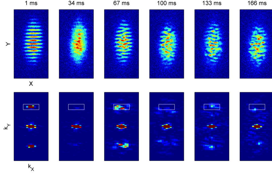
Figure 5.8: Loss of contrast due to vortices. Real space (top) and Fourier space (images) of the 65/ \mu\text{m} pattern in a sample full of vortices. The images are shown roughly every half cycle. The inhomogeneous decay and fringe pattern is due to a large number of vortices produced by condensing the sample too quickly. For instance, the 67 ms image contains roughly a dozen vortices.
