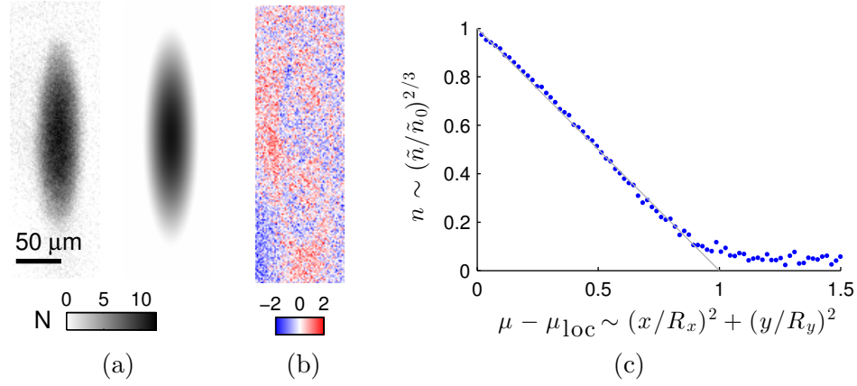
Figure 3.4: Imaging atoms in the surfboard trap. (a) Image (left) and least-squares fit (right) to a Thomas-Fermi profile \tilde{n} = \tilde{n}_0 (1 - x^2/R_x^2 - y^2/R_y^2)^{3/2} of 2 \times 10^4 atoms, approximately 5% of the sample. The scalebar is the number of atoms per 1.6 \mu\text{m} \times 1.6 \mu\text{m} pixel. (b) Residuals may be due to the imaging resolution, anharmonicity of the trap, or nonlinearity in the fit. (c) Density vs chemical potential for a BEC. We integrate the in-plane density n \propto \tilde{n}^{2/3} along elliptical rings of constant local chemical potential \mu_{\text{local}} = \mu - \frac{1}{2}m(\omega_x^2 x^2 + \omega_y y^2) . When plotted in this way, we observe a linear behavior is because of the nonlinear equation of state p = gn^2/2 (in general, \tilde{n} \propto \mu_{\text{local}}^{(\alpha+1)/(2\alpha-2)} for a system with p \propto n^\alpha ). The wings are most likely due to 2-5% thermal atoms, which exhibit a different equation of state, though imaging aberrations distorting the edge of the condensate might contribute.
