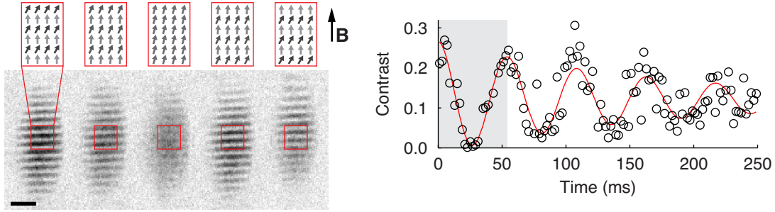
Figure 5.6: Sample images from the contrast interferometer. (Left) The system is initialized with a magnetization that is periodically tilted in the x - z plane (top), where the corresponding density of m_F = 0 atoms is a series of straight fringes. The contrast of the fringes disappear and appear every half cycle. (Right) The contrast of the Fourier transform oscillates at twice the eigenfrequency. The system damps towards a finite contrast, possibly because of inhomogeneous broadening.
