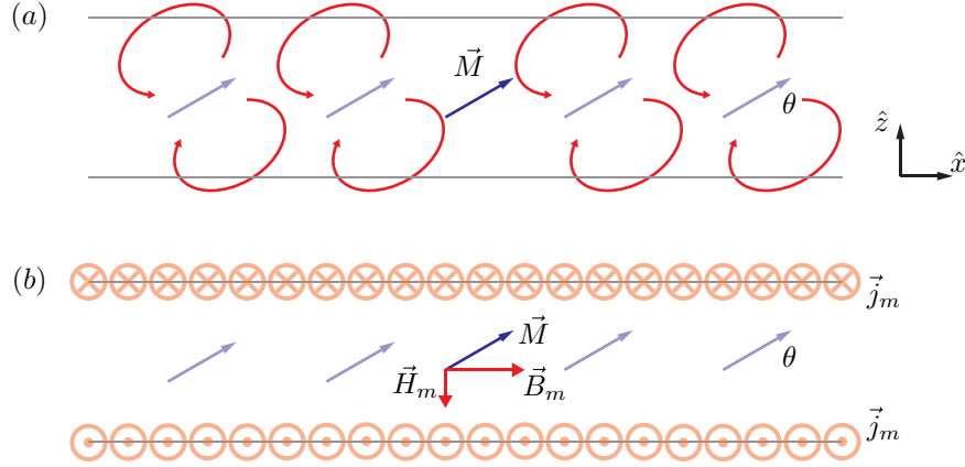
Figure 5.20: Dipolar interaction schematic. (a) A series of spins with magnetization \vec{M} tilted an angle \theta from the plane is equivalent to (b) an effective current density \vec{j}_m , which induces \vec{B}_m and \vec{H}_m fields.
