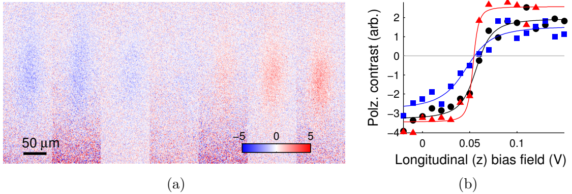
Figure 4.4: Calibrating the magnetic field orientation with polarization contrast imaging. (a) The sign of the polarization contrast signal reverses as the magnetic field is oriented towards or away from the imaging axis z . For an in-plane field, the signal disappears. Each image is taken at a different value of the z component of a magnetic field. (b) We characterize the transverse field and zero the z component of the magnetization by integrating the polarization contrast signal. Each scan corresponds to a different transverse field setting. The light level is sufficient to destroy the sample, despite the meager signal-to-noise. These images are taken detuned +80 MHz from the D2, F = 1 \rightarrow F' = 2 transition.
