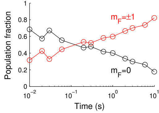
Figure 4.22: Spin populations during a quench. The initial imbalance between m_F = 0 and m_F = \pm 1 is set by a brief rf pulse that uniformly rotates a uniform (0, 1, 0) ground state. During the quench to the ferromagnetic state, the m_F = 0 slowly vanishes.
